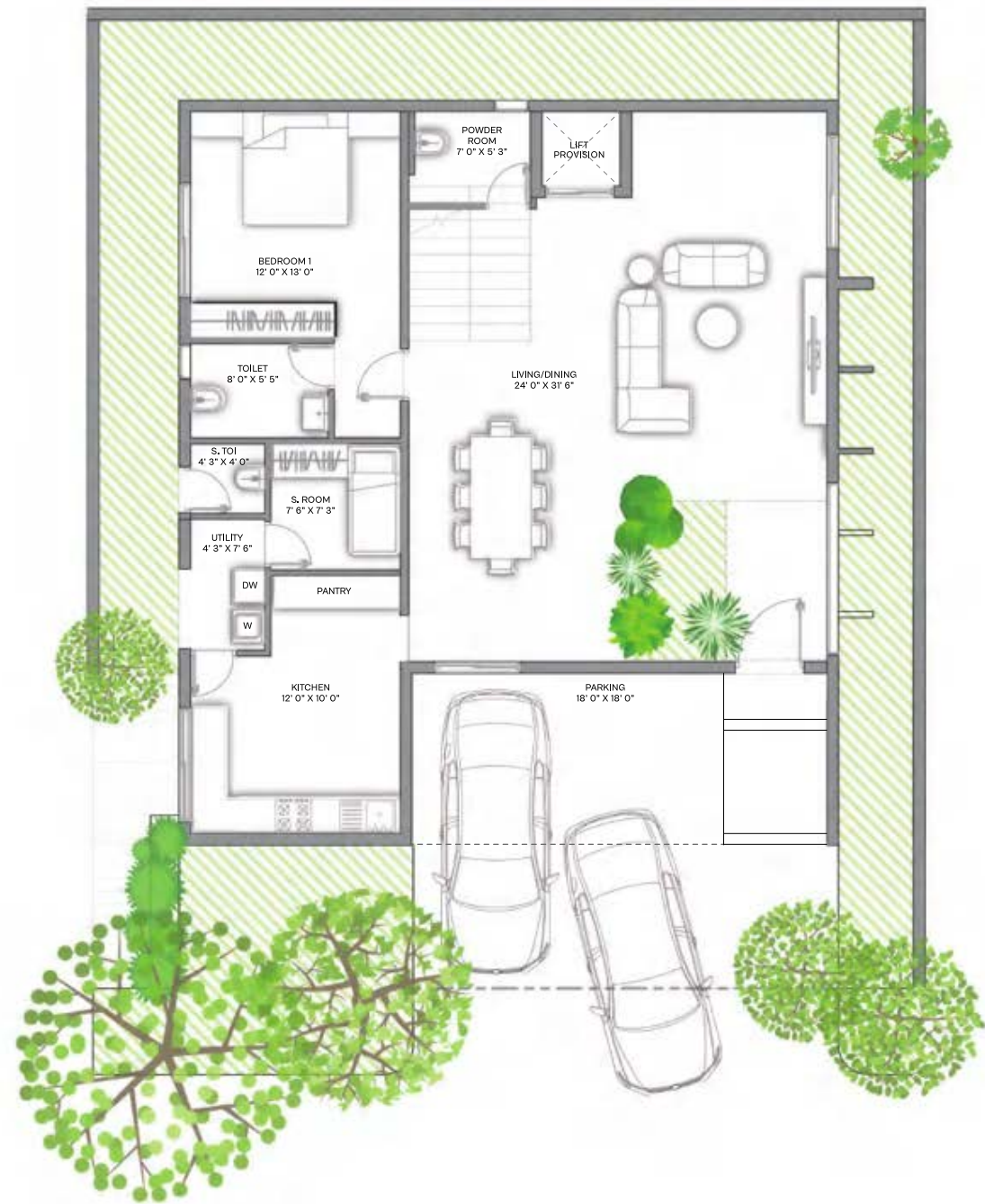
Ground Floor ▲
